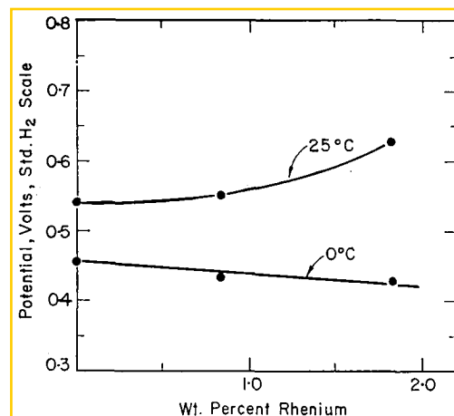
Fig. 2. Critical pitting potentials of 18%Cr, 10%Ni, Re stainless steels in 0.1N NaBr
