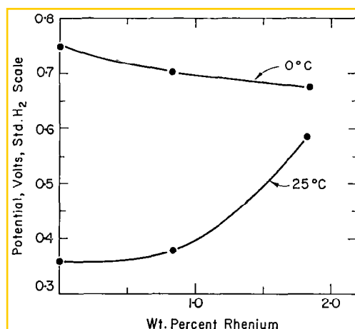
FIG. 1. Critical pitting potentials of 18%Cr, 10%Ni, Re stainless steels in 0.1N NaCl.
